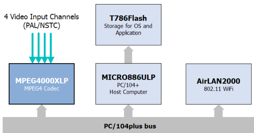
Wireless Video Telemetry System
