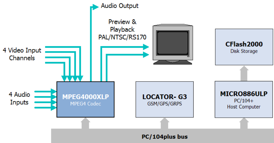
Mobile MPEG-4 Record and Playback System
