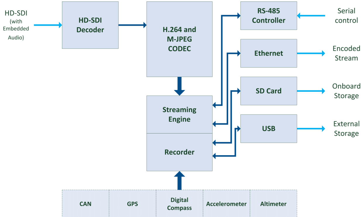
StreamCorder-HD-SDI Functional Diagram
