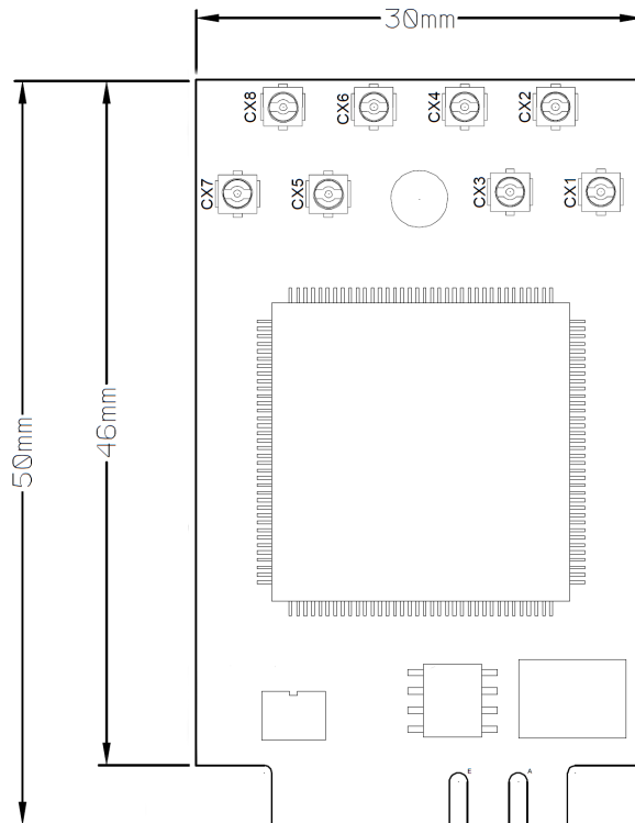
AVC8000M2 Mechanical Drawing
