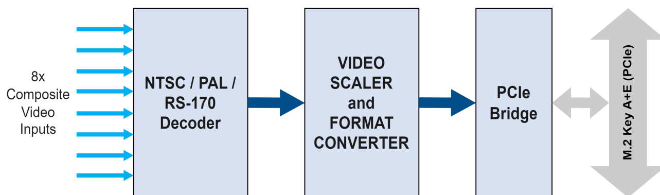
AVC8000M2 Functional Diagram
