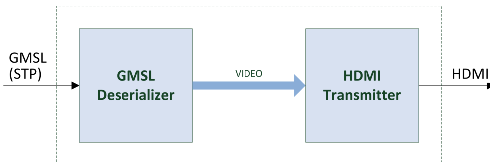
nanoGMSL2HDMI Functional Diagram
